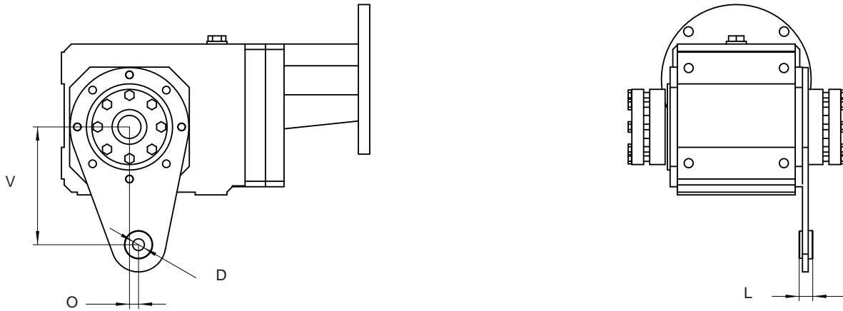
Drawing for Units KSS102 — KSS303
